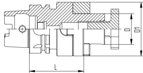
Croquis 2 HSK-A/KFD
