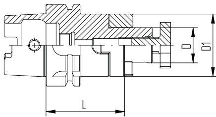
Croquis 1 HSK-A/KFD
